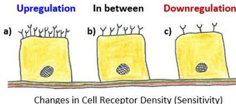
Figure 8.12 Shows the receptor density (sensitivity) changing on the cell surface, as it will always do in response to variations in levels of stimulation. In a) there is an upregulation of surface receptors due to a reduction of a signal molecule stimulus. In c) there is a downregulation of surface receptors due to overstimulation by the signal molecule. The cell in b) is in a transient state in between a) and c) and the direction it will move will be influenced by the amount of the ligand (signal molecule) present.
