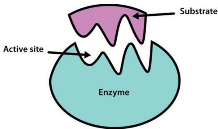
Figure 3.1 Seen here is a diagram of an enzyme, showing its active site where it can bind with a substrate (the substance being acted on by the enzyme) and speed up the chemical reaction.
