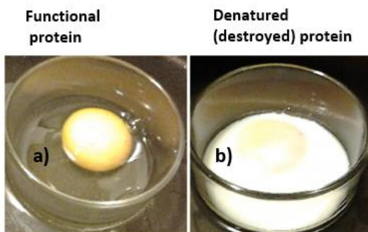
Figure 3.6 In the bowl a) on the left, the albumin portion of an egg (the egg white) is raw and has a viscous, slippery texture which is transparent. When this is heated up to 184^{\circ}\text{F} it changes into b) a rubbery white texture.
