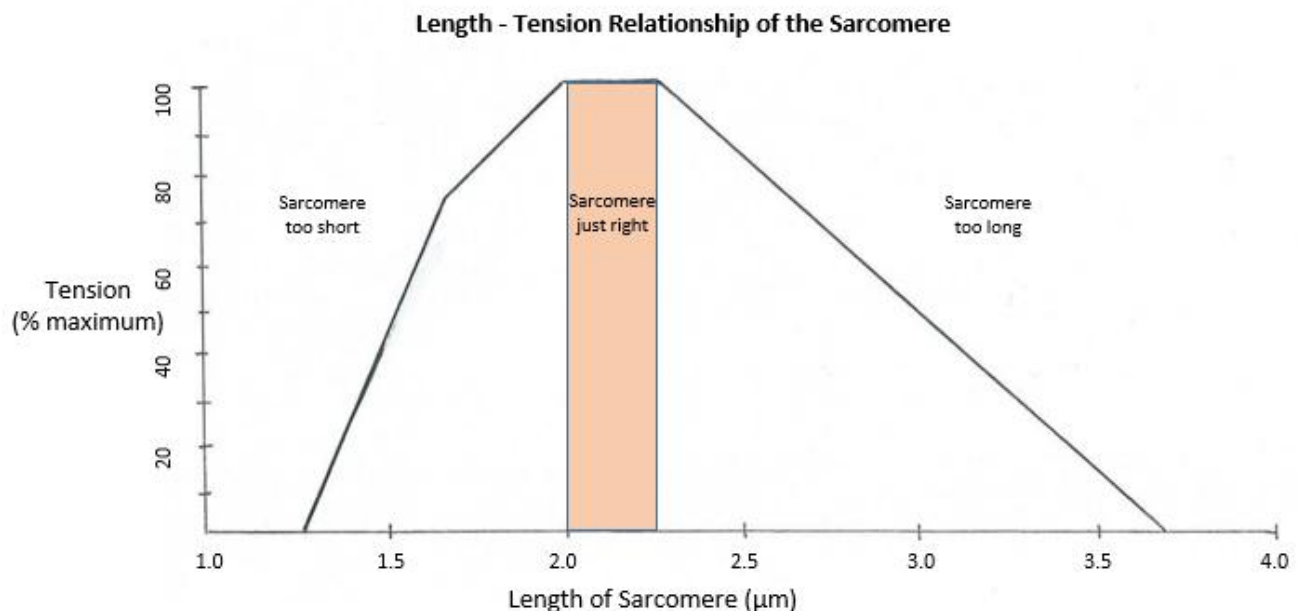
Figure 13.18 This graph shows the amount of tension generated (as a percentage of the maximum) when a sarcomere is stimulated at various 'resting' lengths in microns ( \mu\text{m} ). The shaded area is the resting sarcomere length that generates the greatest amount of tension (force) and this is called the 'optimal length'. When the sarcomere is at the length when contraction is stimulated, it generates the greatest amount of force. When the sarcomere is too short (left side of optimal length) or too long (right side of optimal length), the sarcomere cannot generate as much tension.
