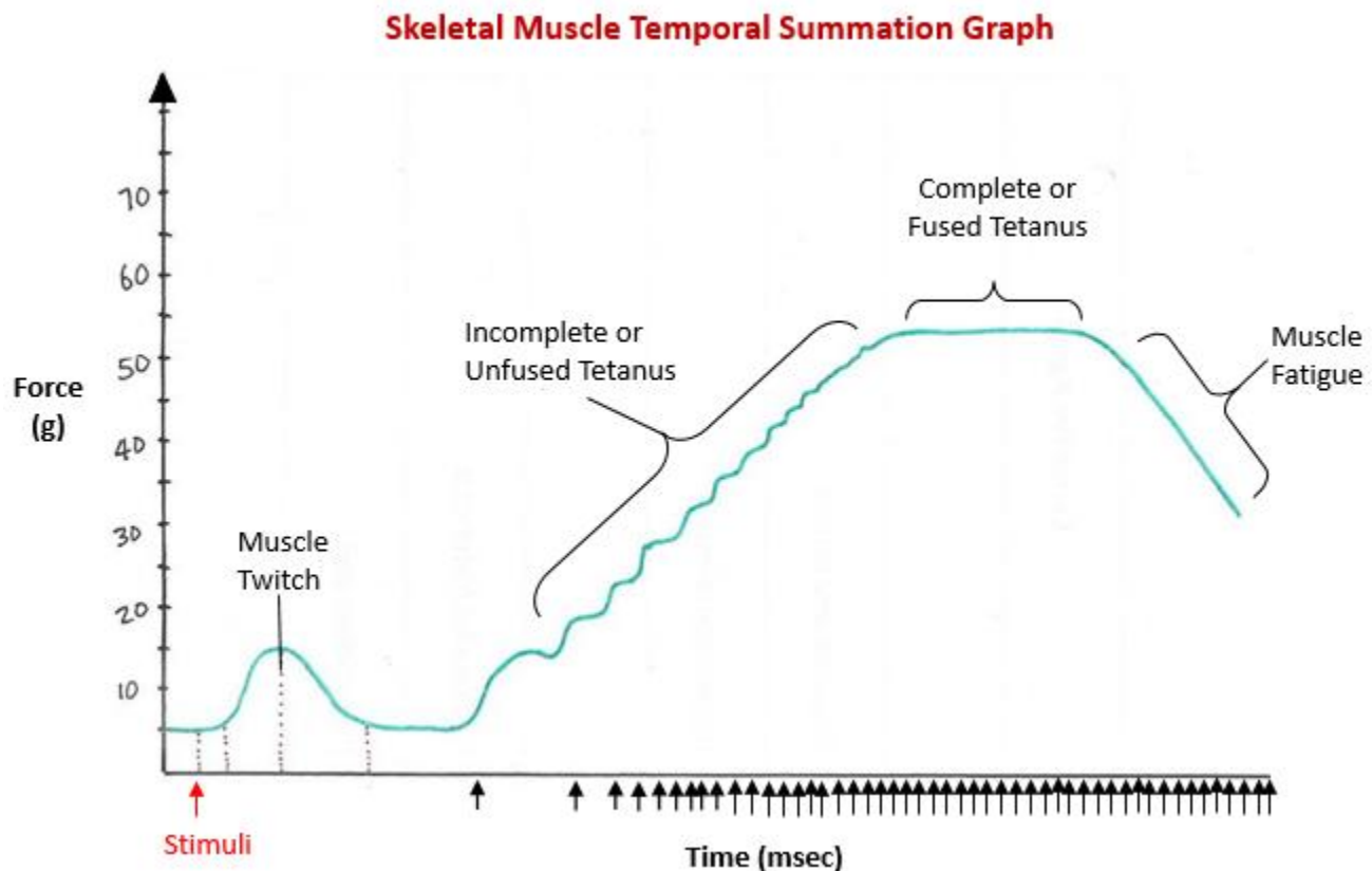
Figure 13.15 This graph shows the changes in force (g) generated during a simple muscle twitch of a single muscle fiber. It then shows how force increases as the frequency of stimulation increased, until maximum tension is reached at complete tetanus. Ultimately, skeletal muscle will fatigue and be unable to sustain tension due to overuse, regardless of stimulation.
