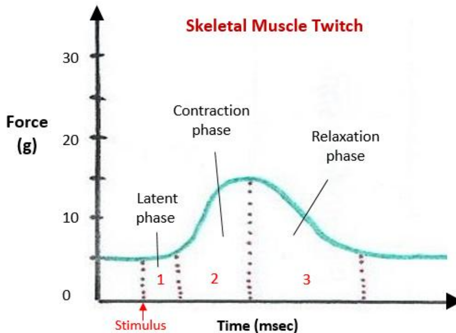
Figure 13.14 This graph shows the changes in force (g) generated during a simple muscle twitch of a single muscle fiber. The muscle twitch has three phases, which are indicated in the graph. First is the latent phase, this is the delay in time from the stimulus until the onset of contraction (shown by the increase in force). Second is the contraction phase when the muscle is generating force (and graph is going up). Third is the relaxation phase when the muscle is no longer generating tension and starts to relax, causing decrease in force.
