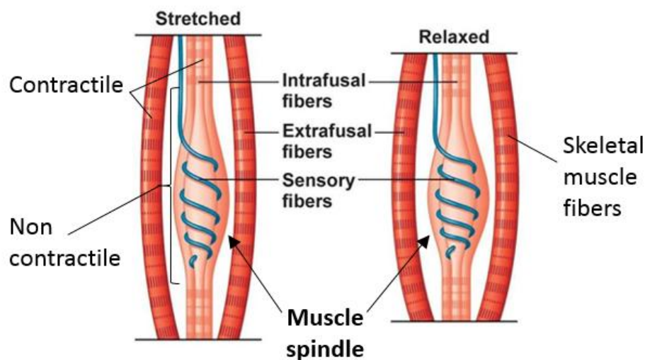
Figure 13.21 Shows the location and structure of the muscle spindle within skeletal muscle. The sensory nerve ending coils around the swollen spindle-shaped connective tissue sac, with intrafusal fibers at both ends, which can contract, but the central swollen area cannot contract. The extrafusal fibers are skeletal muscle fibers that are not a part of the muscle spindle unit.
