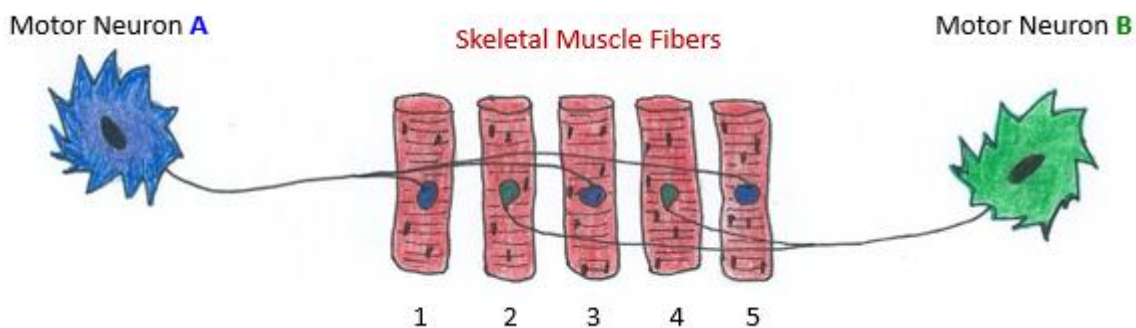
Figure 13.16 In the drawing above there are two skeletal motor units, A and B. Motor Unit A is motor neuron A and muscle fibers 1, 3 and 5. Motor unit B is motor neuron B and muscle fibers 2 and 4. Motor units can range from being very small to very large. In any one motor unit the muscles fibers must all be the same type, that is slow, intermediate or fast twitch skeletal muscle fibers.
